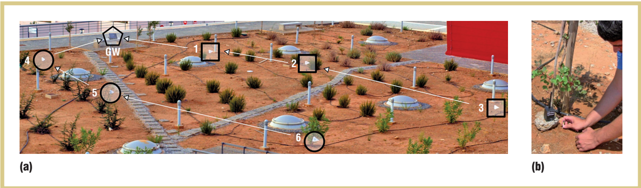
Figure 7. The wireless network deployed outdoors for demonstration purposes. It has (a) two chains (chain 1 in rectangles and chain 2 in circles) and seven nodes and (b) a soil wetness sensor. No special iCube mounting was performed.
